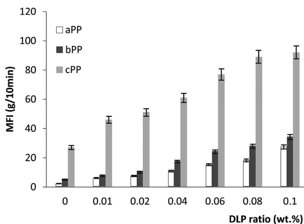
Figure 1. Melt flow index values of PP matrices.
