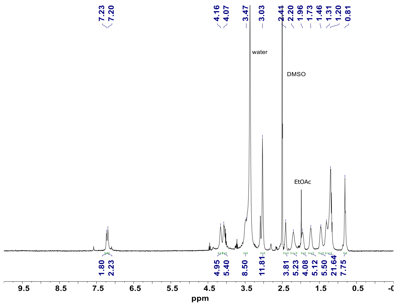
Figure S4. ^1\text{H} NMR spectrum of P2 in \text{DMSO-d}_6 .
