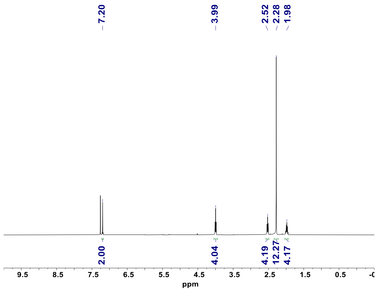
Figure S2. 1 H NMR spectrum of 3 in CDCl 3 .
