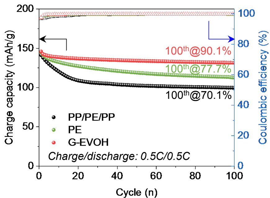
Figure S1 Comparison of the cycling performance with LCO|Graphite full cells at 0.5C rate.
