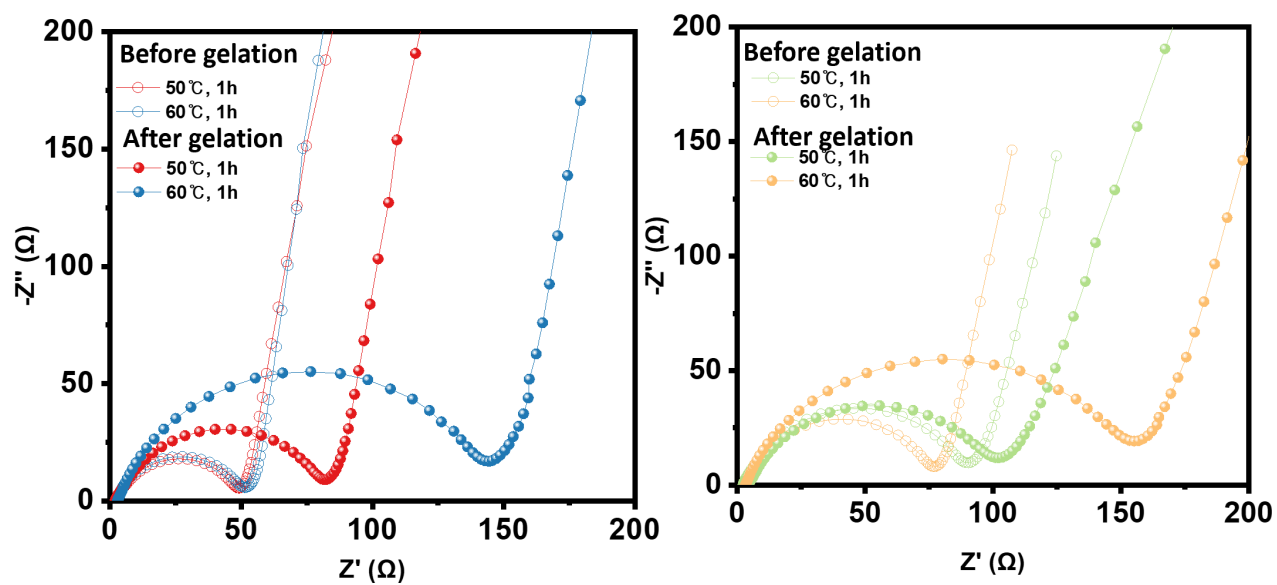
Figure S1. Nyquist plot of quasi-solid electrolyte: (a) NCM811 | PEGDA 4 wt.% | Li; (b) NCM811 | PEGDA 8 wt.% | Li
